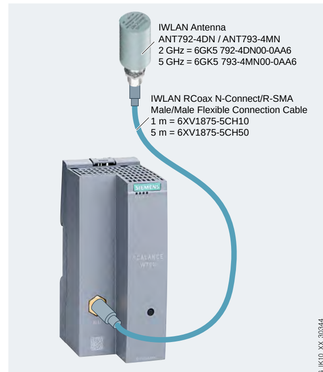
Client Module SCALANCE W722-1 RJ45
