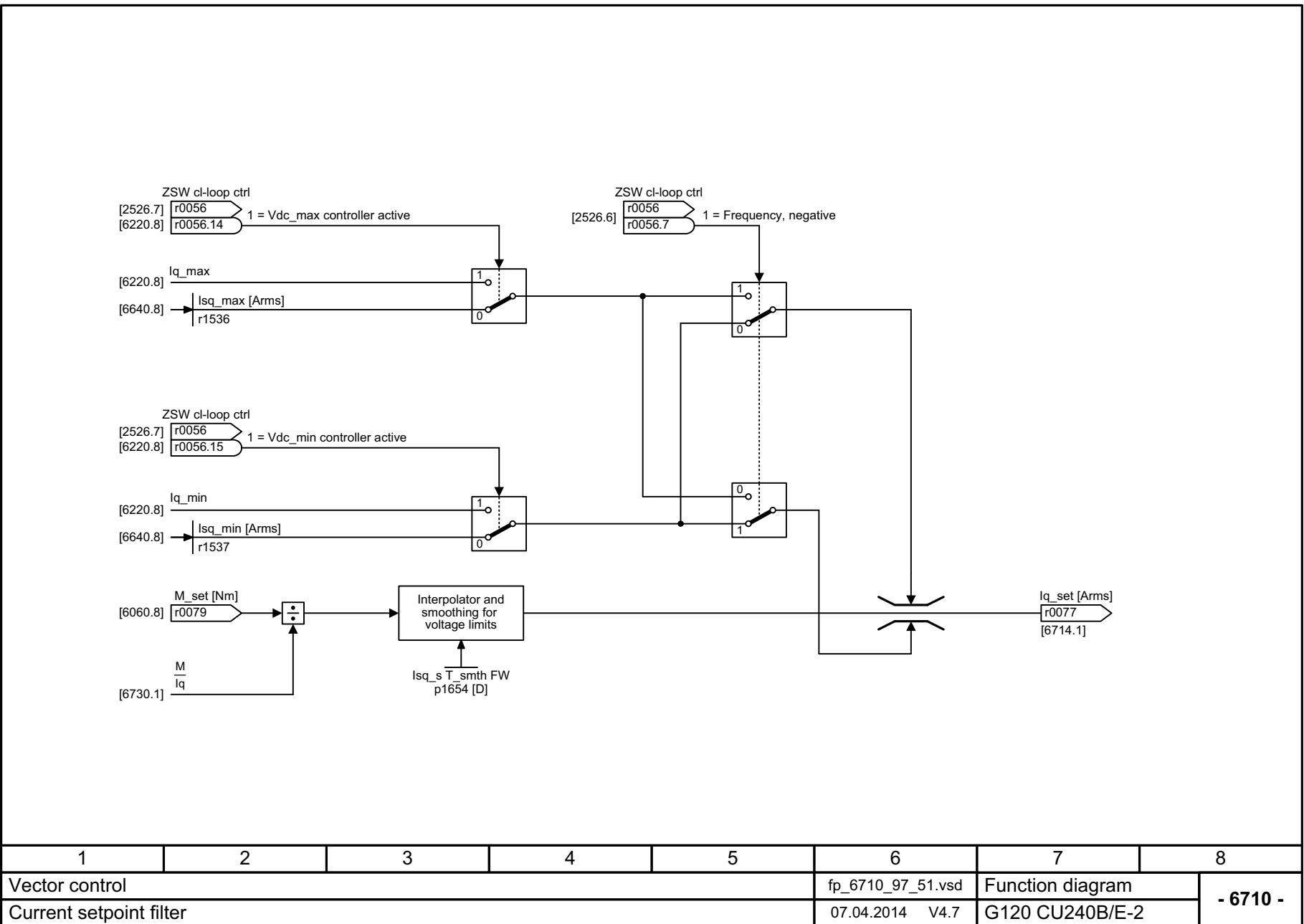
Fig. 3-101 6710 – Current setpoint filter
