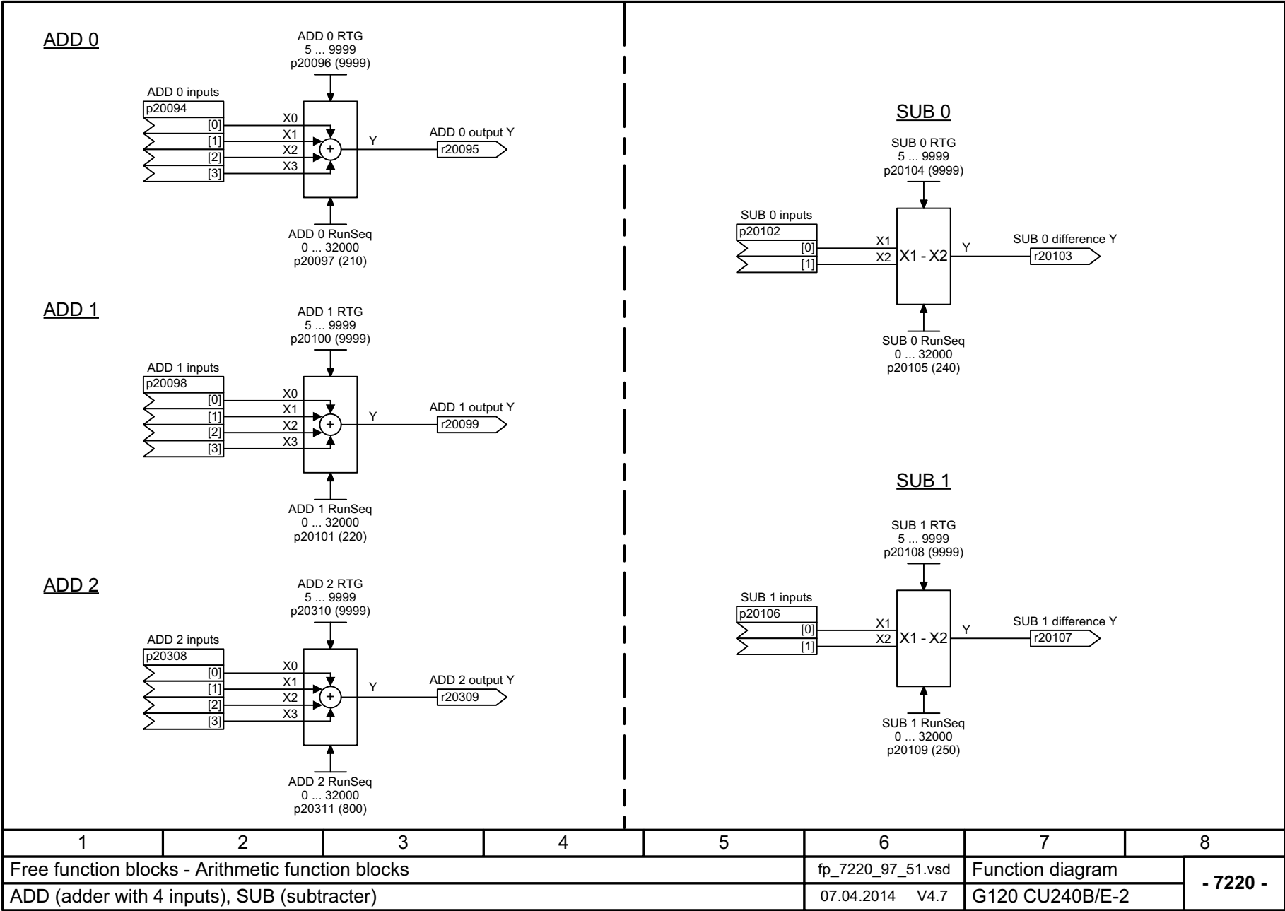
Fig. 3-116 7220 – ADD (adder with 4 inputs), SUB (subtractor)
