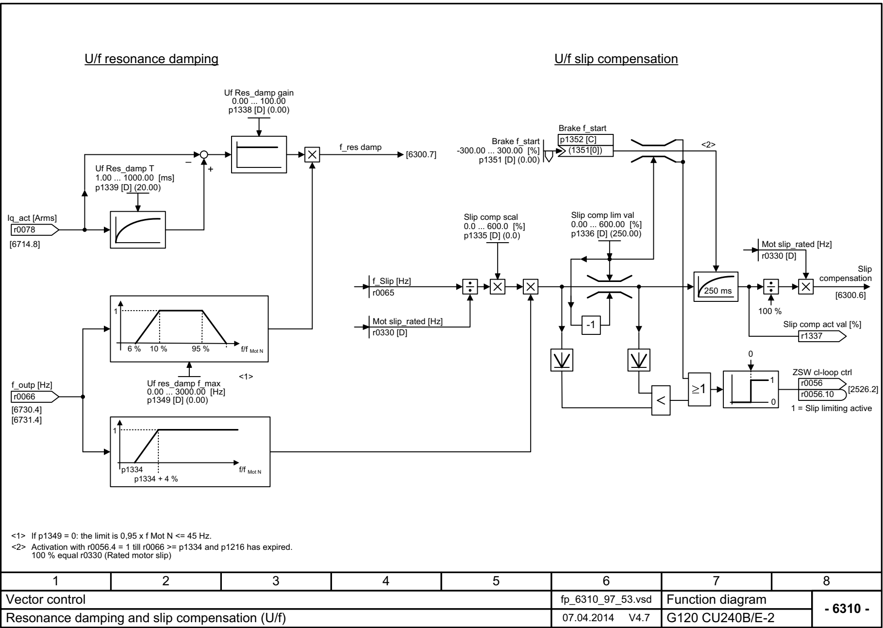
Fig. 3-94 6310 – Resonance damping and slip compensation (U/f)
