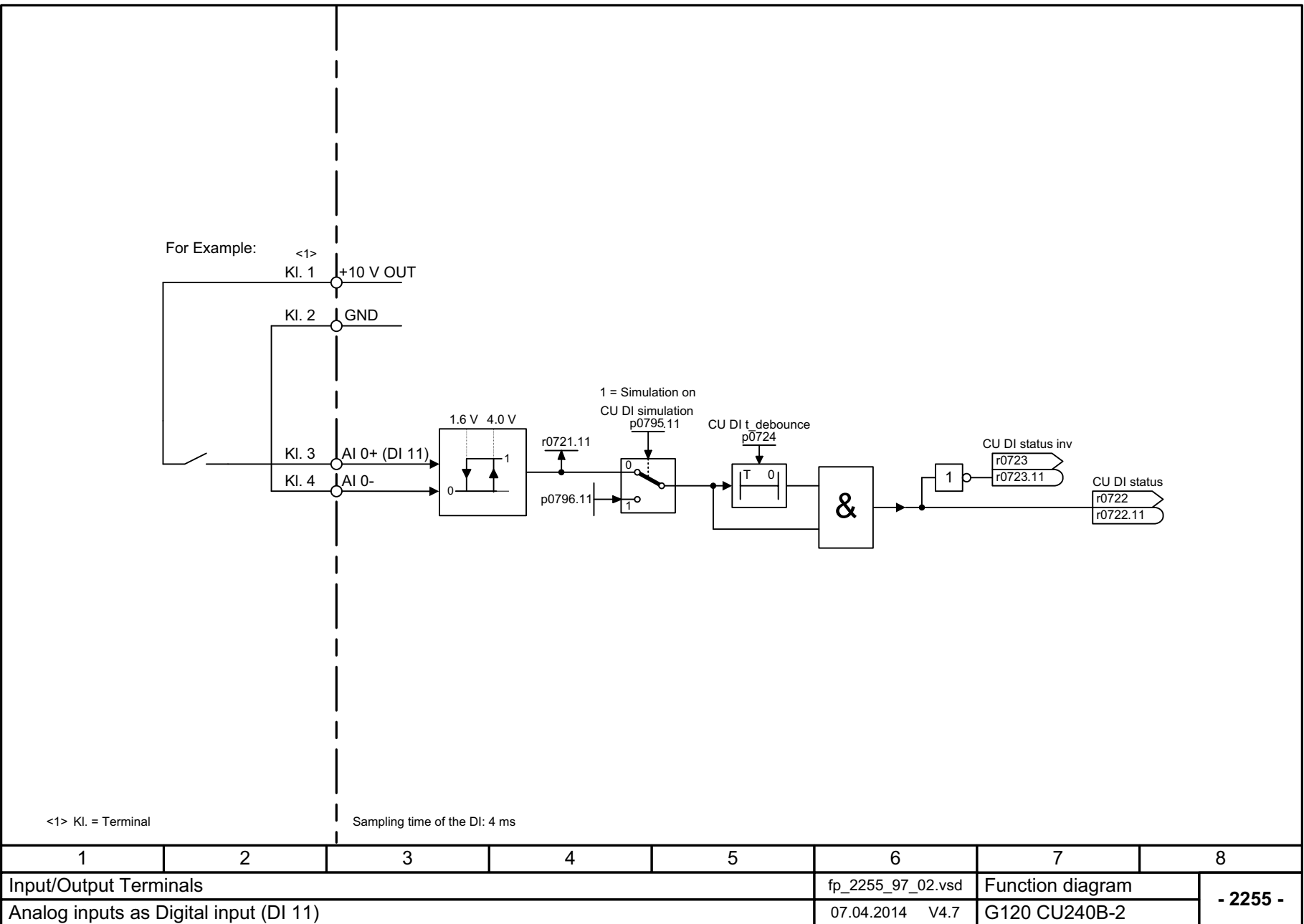
Fig. 3-13 2255 – CU240B-2: Analog inputs as digital inputs (DI 11)
