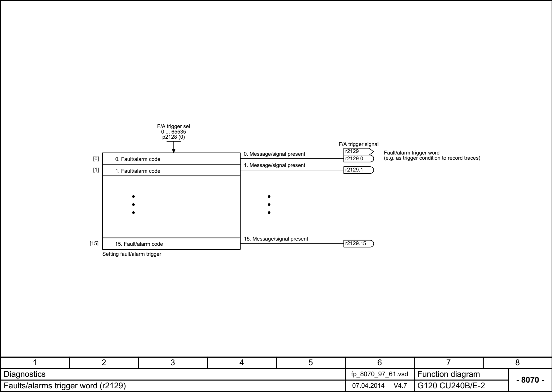
Fig. 3-148 8070 – Faults/alarms trigger word (r2129)
