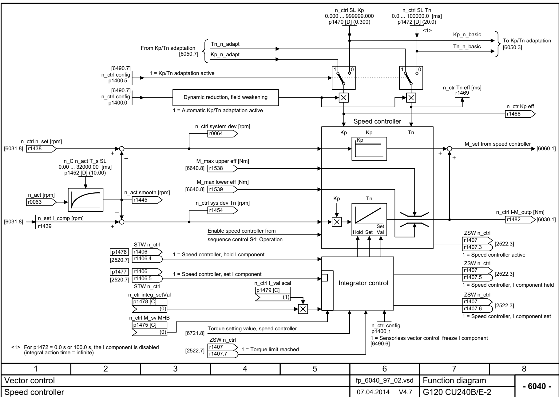
Fig. 3-88 6040 – Speed controller
