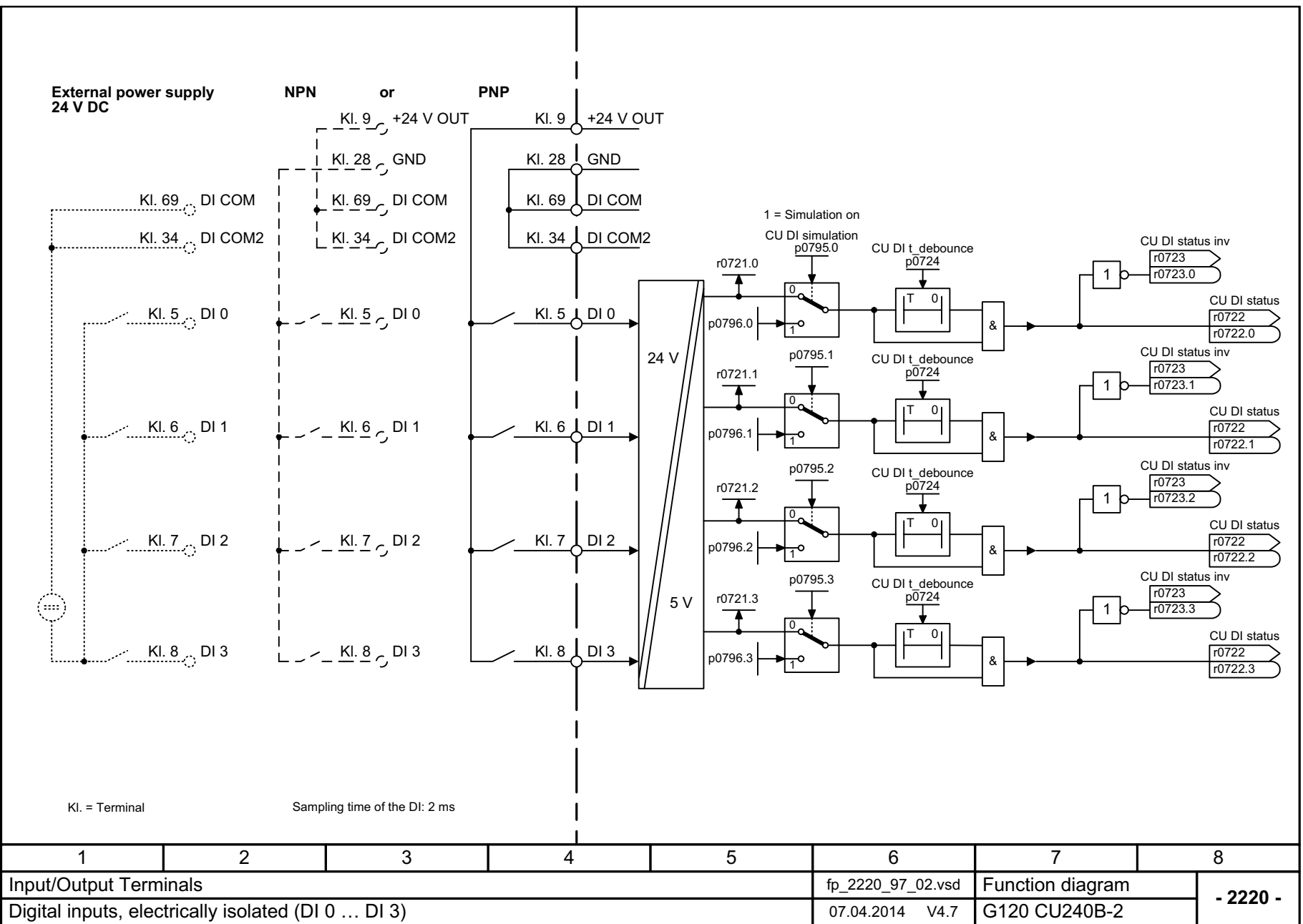
Fig. 3-7 2220 – CU240B-2: Digital inputs, electrically isolated (DI 0 ... DI 3)
