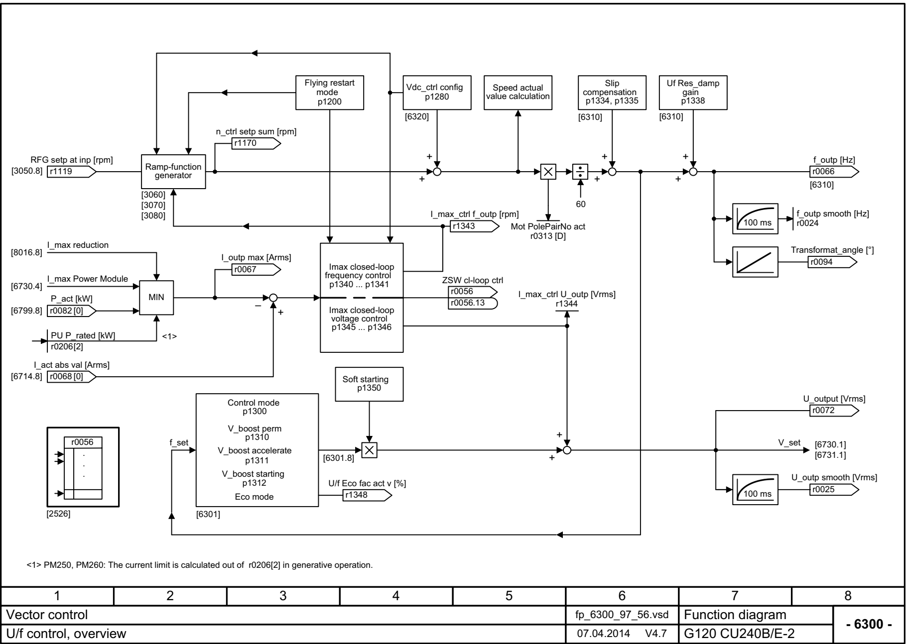
Fig. 3-92 6300 – U/f control, overview
