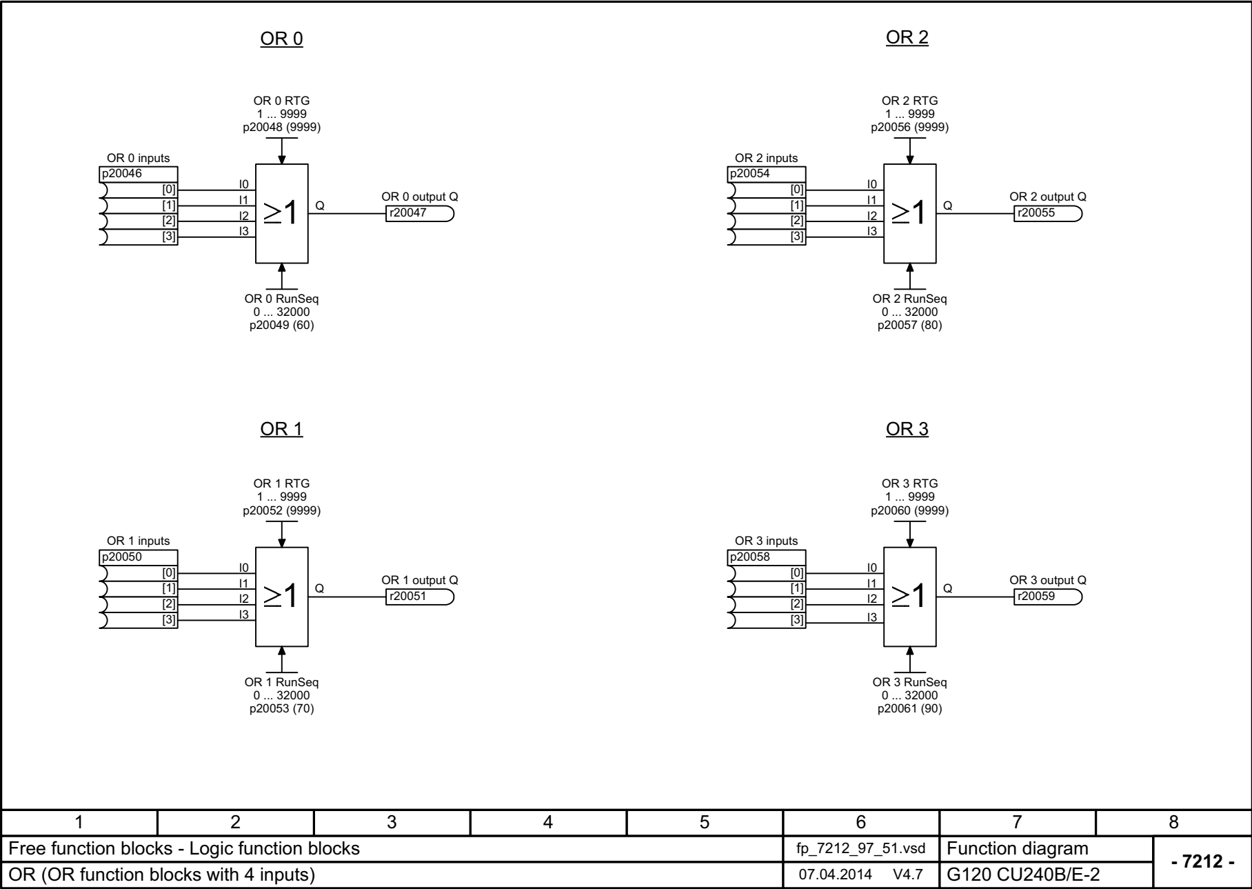
Fig. 3-113 7212 – OR (OR function blocks with 4 inputs)
