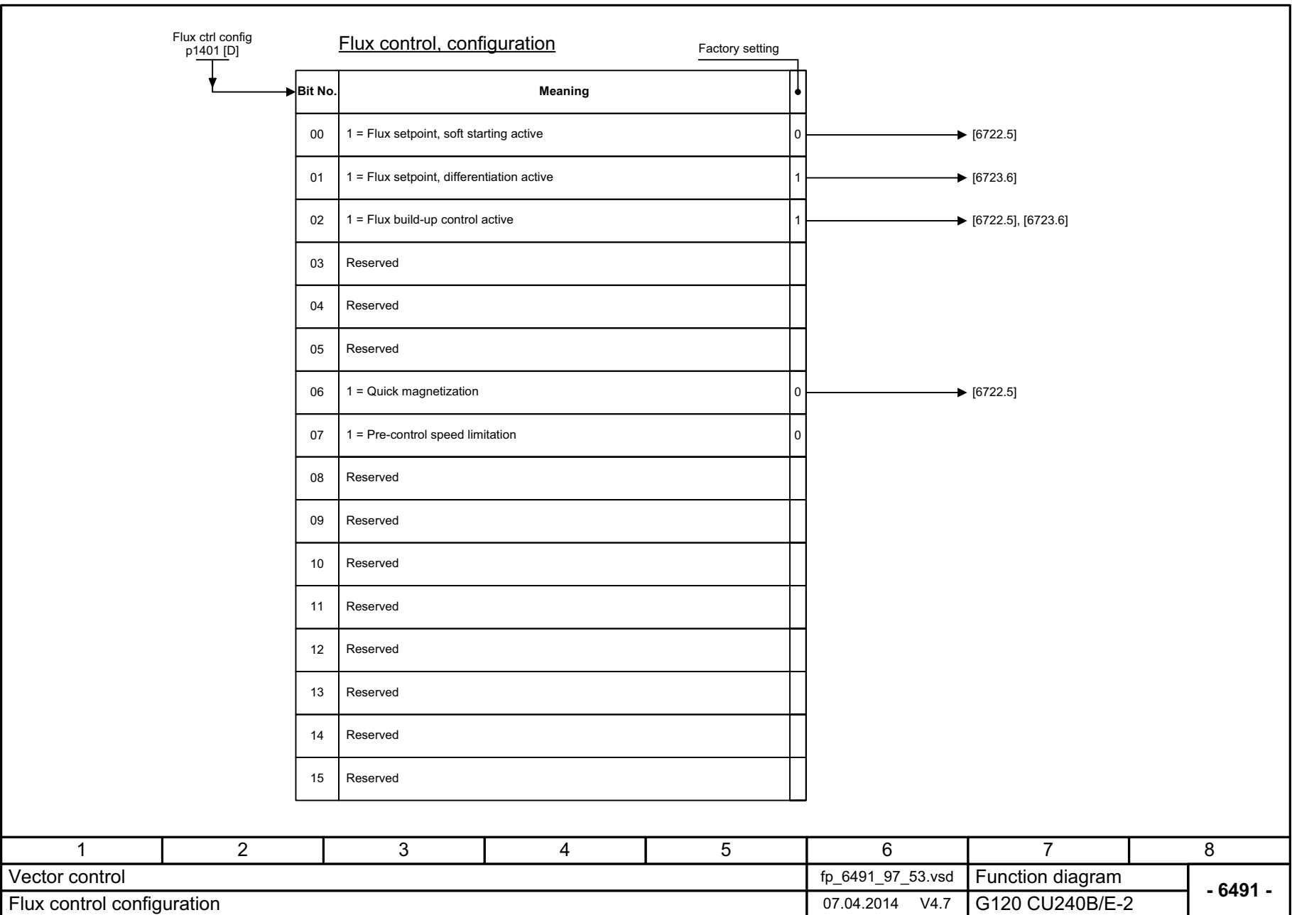
Fig. 3-97 6491 – Flux control configuration
