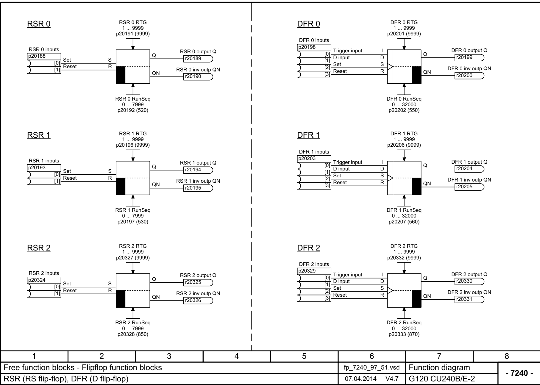
Fig. 3-125 7240 – RSR (RS flip-flop), DFR (D flip-flop)
