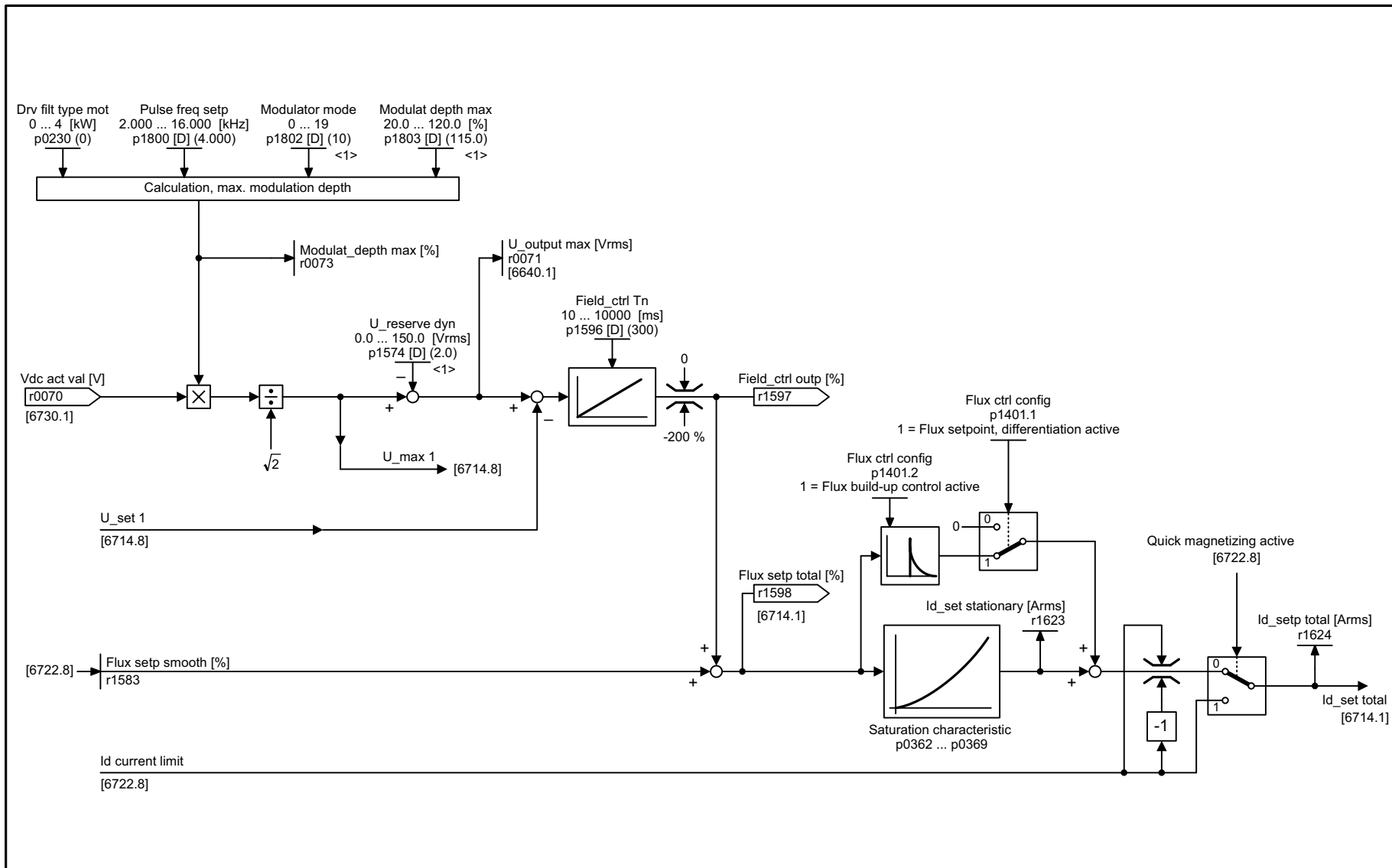
Fig. 3-105 6723 – Field weakening controller, flux controller (ASM, p0300 = 1)
