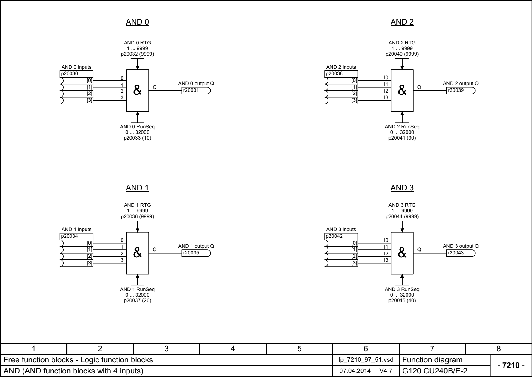
Fig. 3-112 7210 – AND (AND function blocks with 4 inputs)
