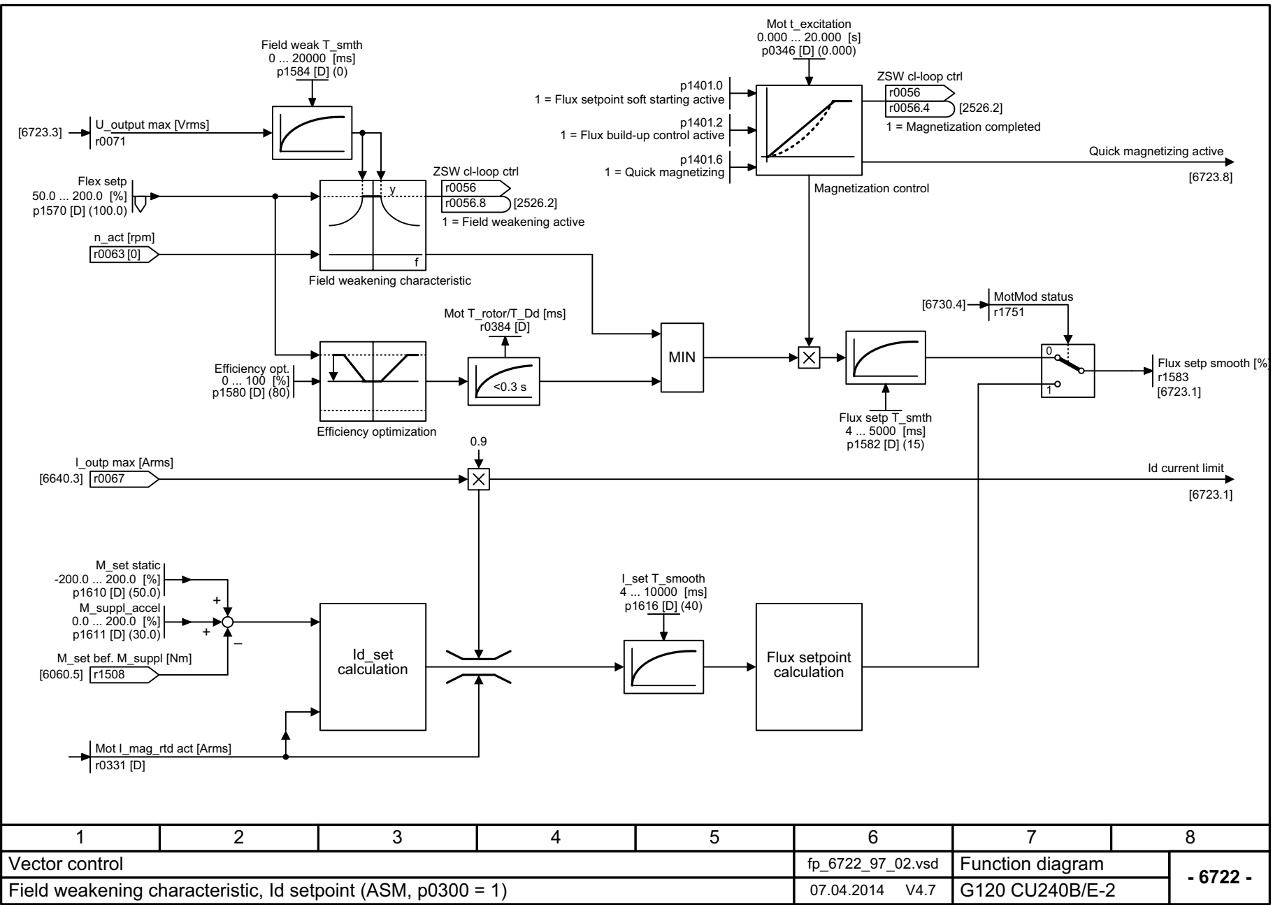
Fig. 3-104 6722 – Field weakening characteristic, Id setpoint (ASM, p0300 = 1)
