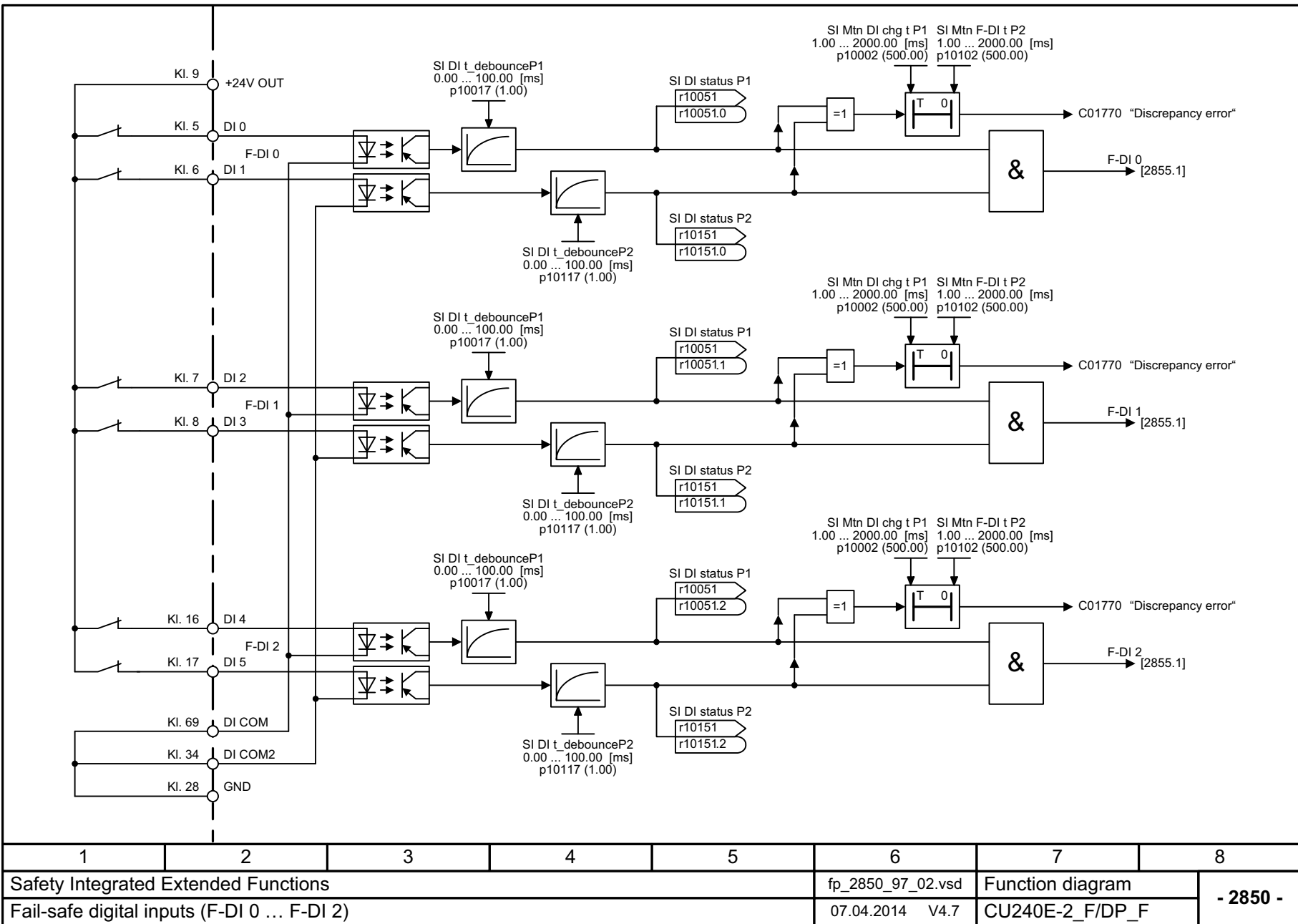
Fig. 3-70 2850 – Fail-safe digital inputs (F-DI 0 ... F-DI 2)
