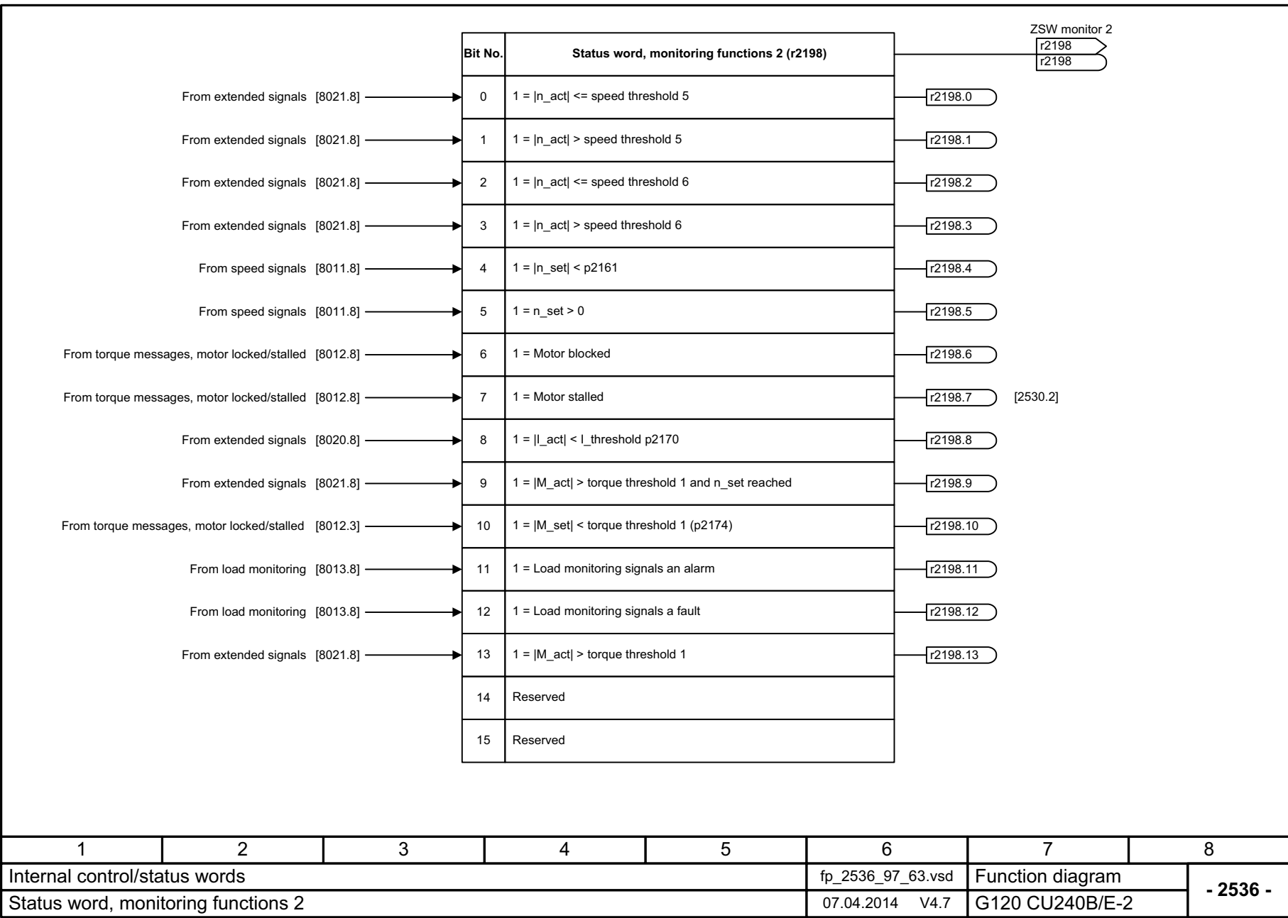
Fig. 3-53 2536 – Status word, monitoring functions 2
