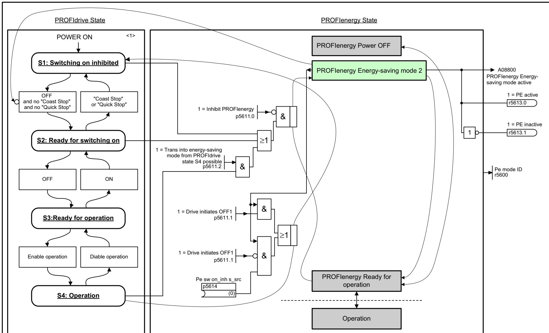
<1> Excerpt from: Basic state machine of a PROFdrive drive axis, source: PROFIBUS Nutzerorganisation (PNO)
