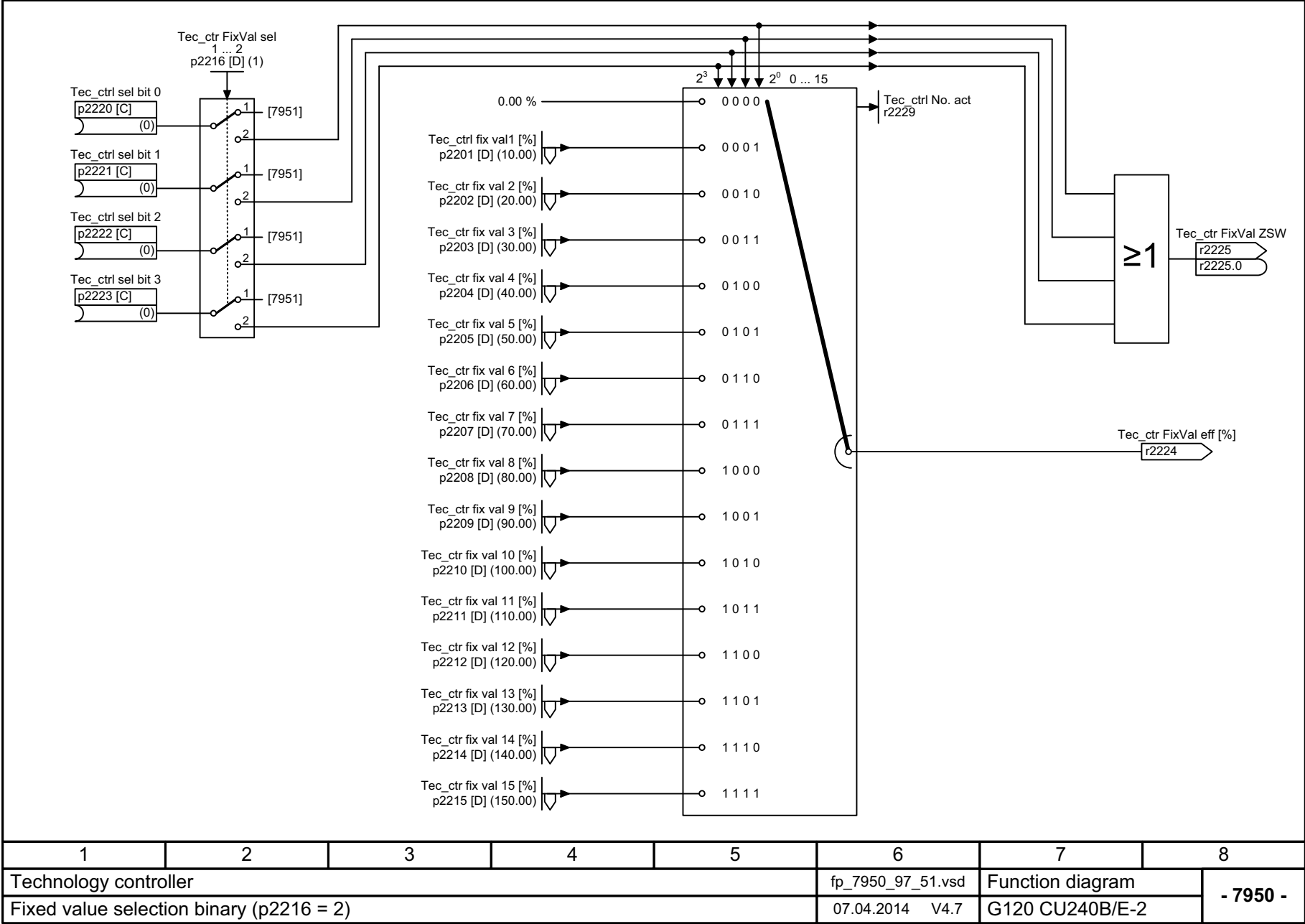
Fig. 3-131 7950 – Fixed value selection binary (p2216 = 2)
