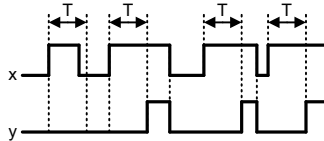
Fig. 3-3 1022 – Explanation of the symbols (part 3)
