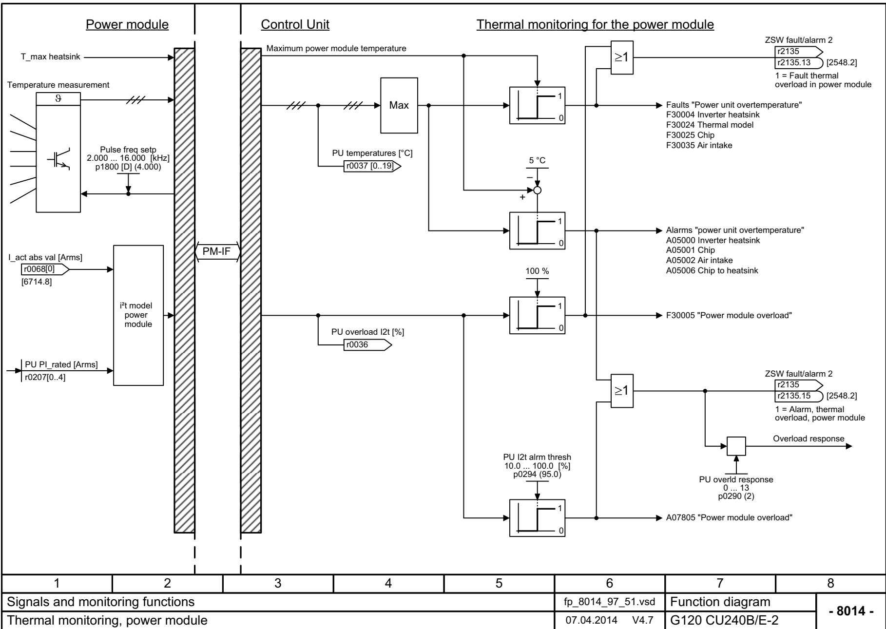
Fig. 3-140 8014 – Thermal monitoring, power unit
