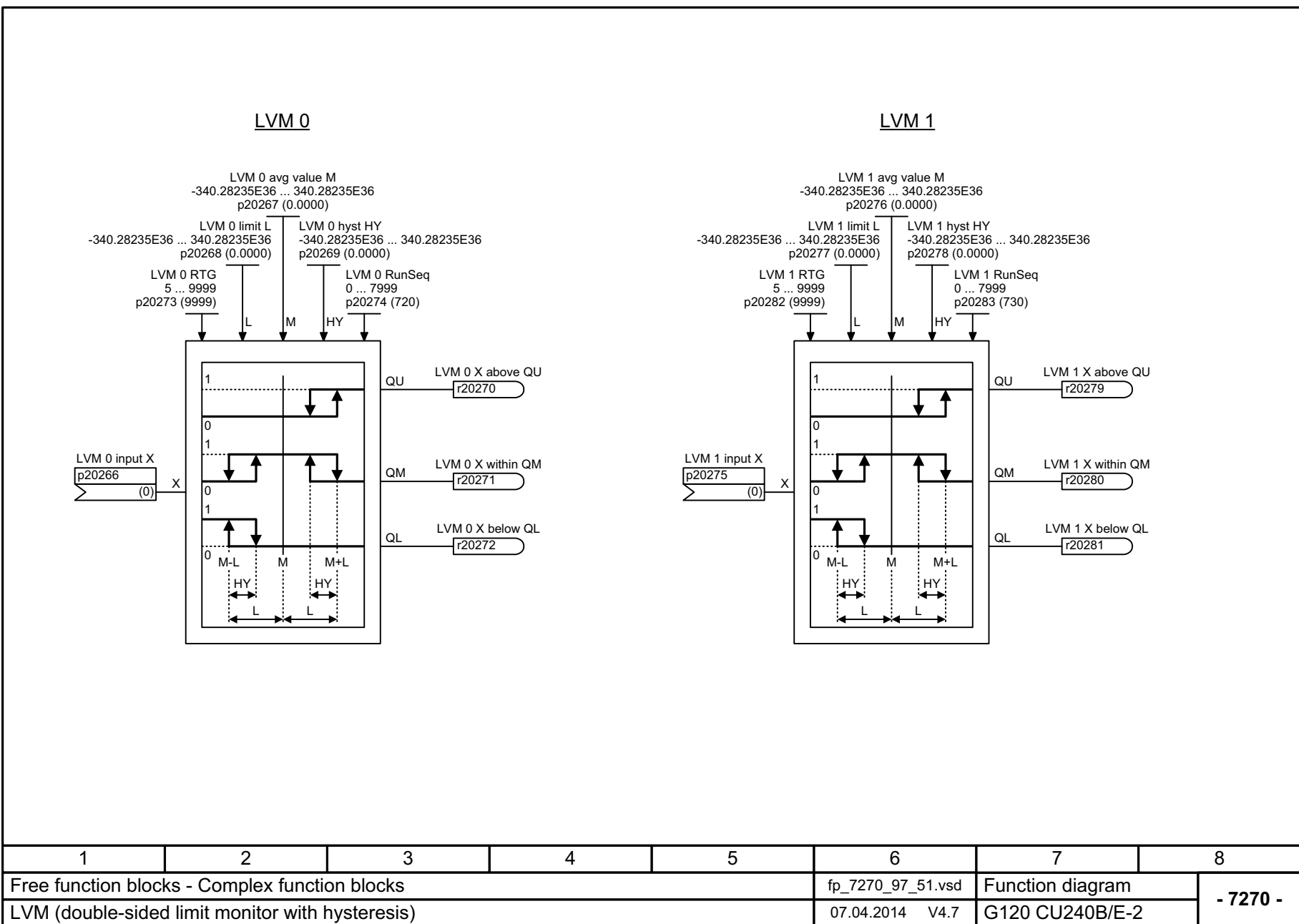
Fig. 3-130 7270 – LVM (double-sided limit monitor with hysteresis)
