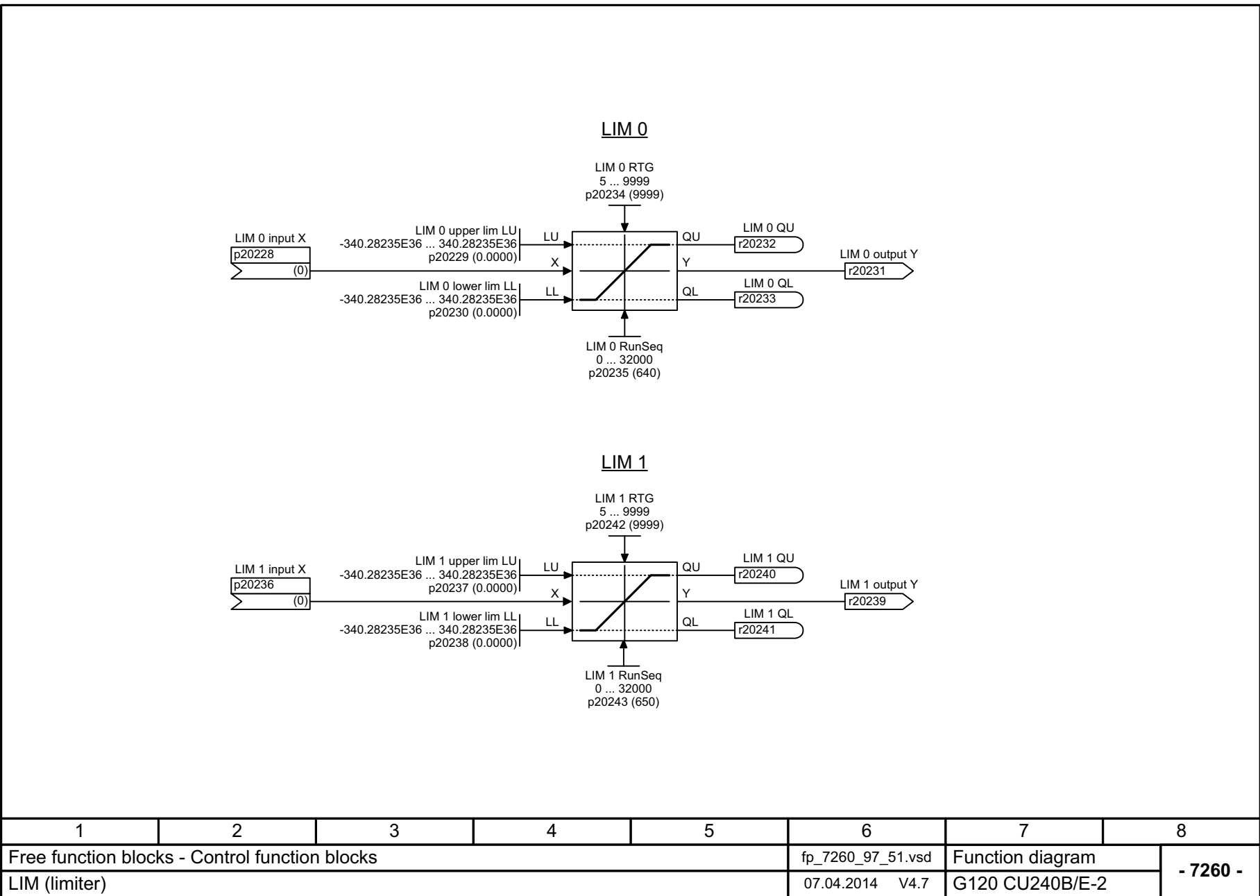
Fig. 3-127 7260 – LIM (limiter)
