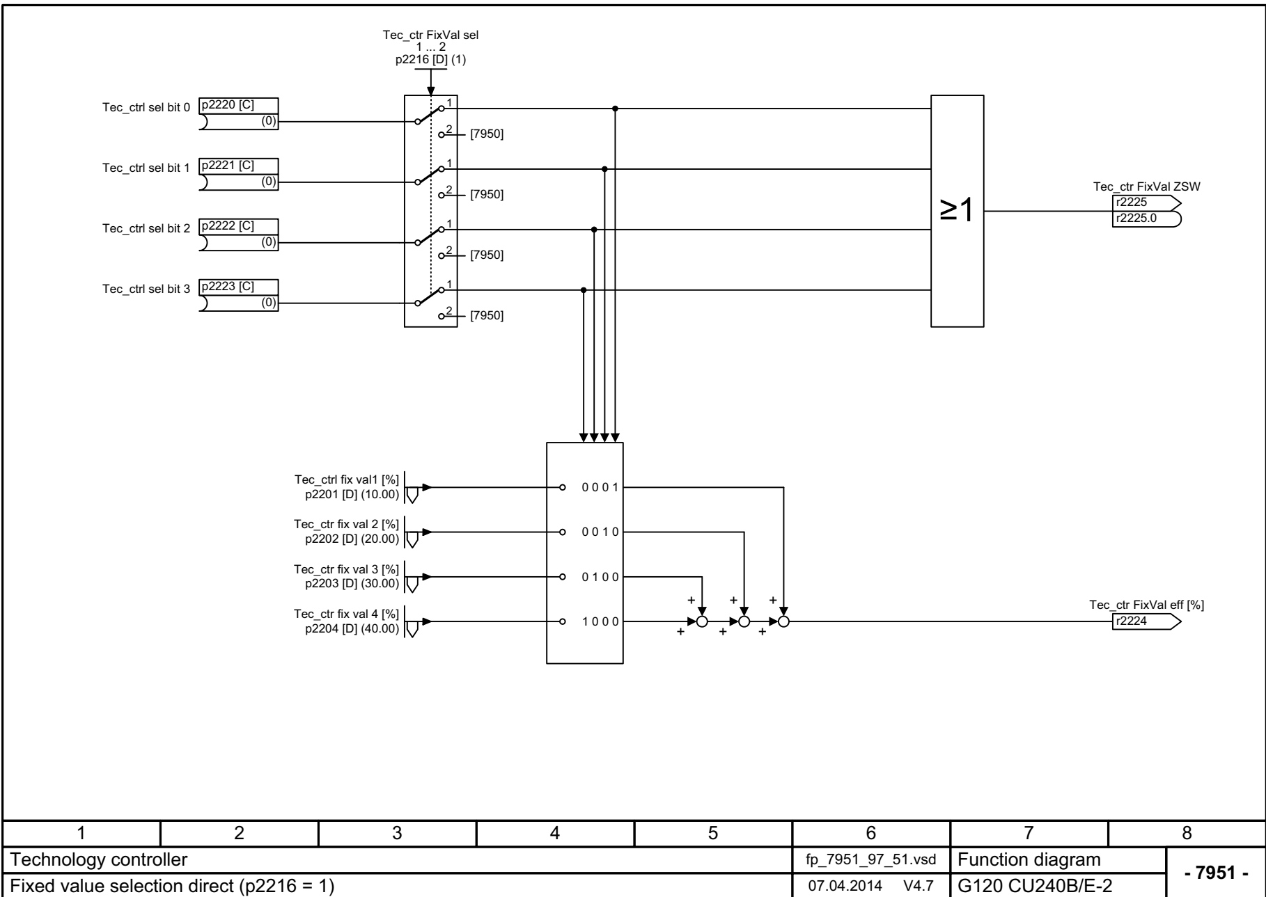
Fig. 3-132 7951 – Fixed value selection direct (p2216 = 1)
