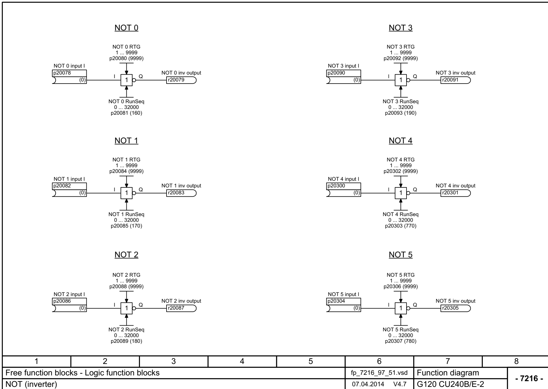
Fig. 3-115 7216 – NOT (inverter) SINAMICS G120 Control Units CU240B-2/CU240E-2 List Manual (LH11), 04/2014, A5E33839529B AA
