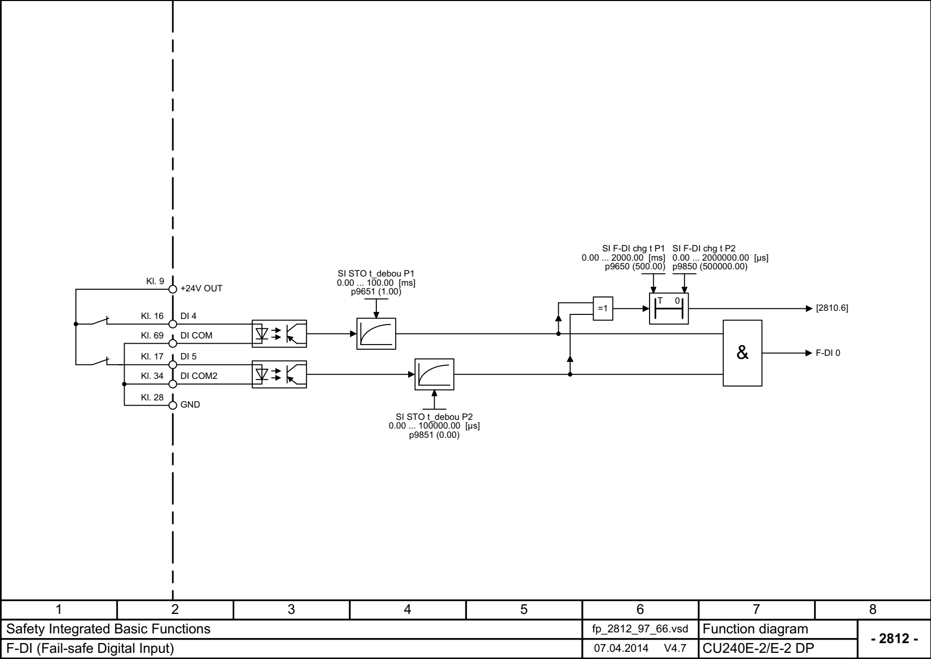
Fig. 3-64 2812 – F-DI (Fail-safe Digital Input)
