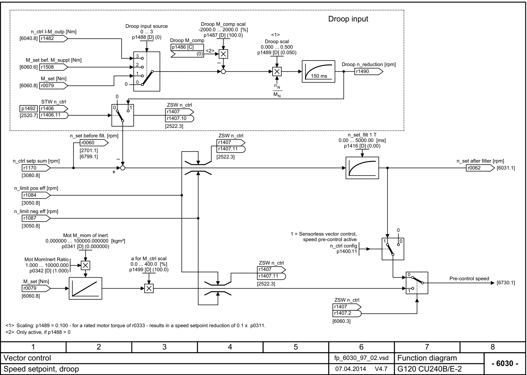
Fig. 3-86 6030 – Speed setpoint, droop
