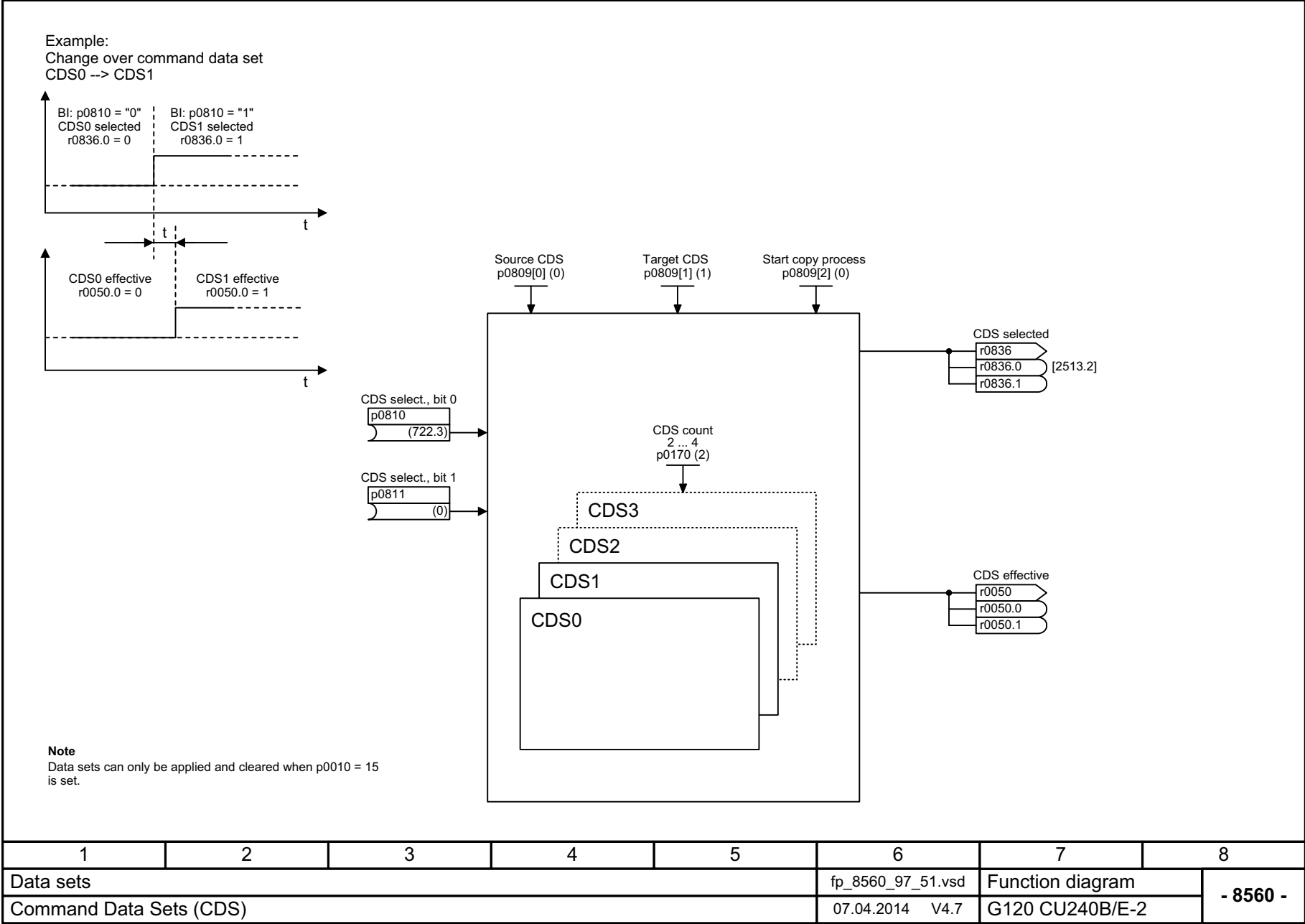
Fig. 3-150 8560 – Command Data Sets (CDS)
