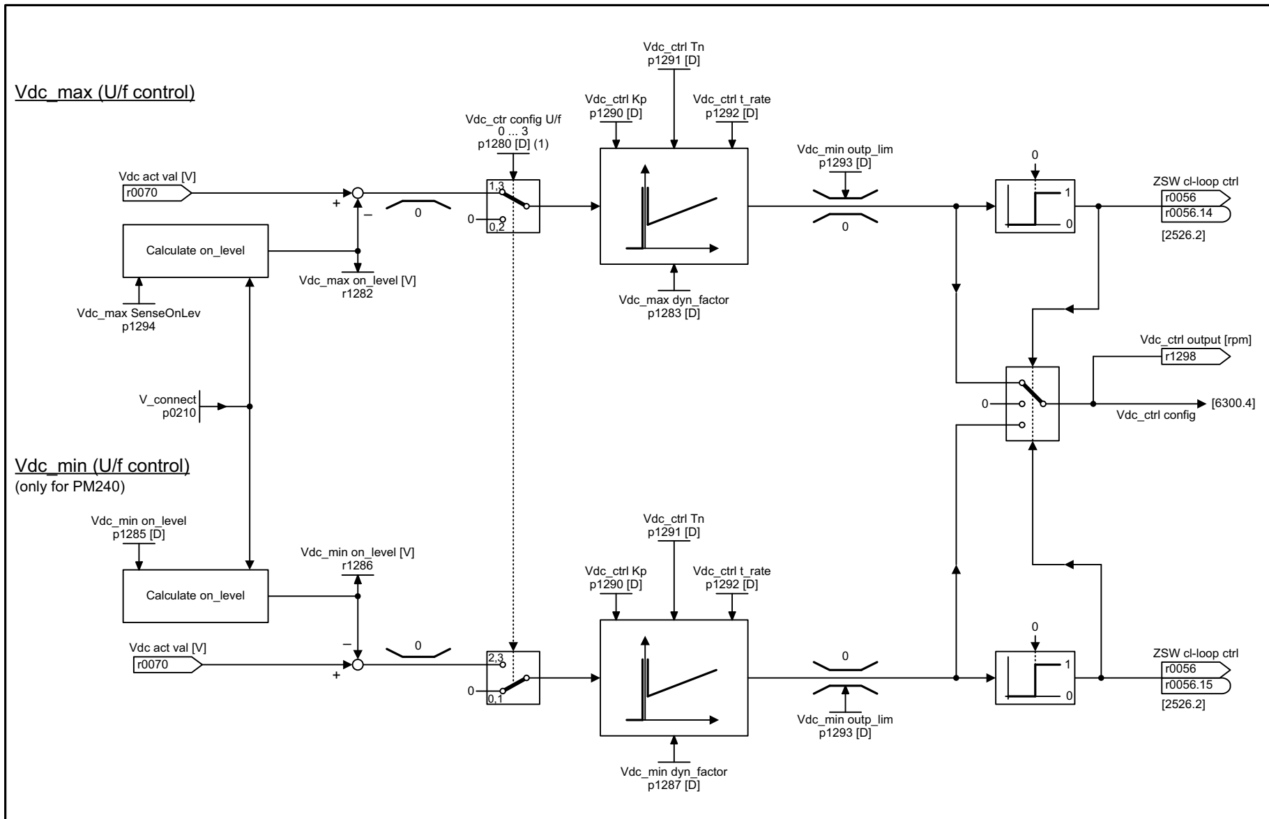
Fig. 3-95 6320 – Vdc_max controller and Vdc_min controller (PM230/PM240), (U/f)
