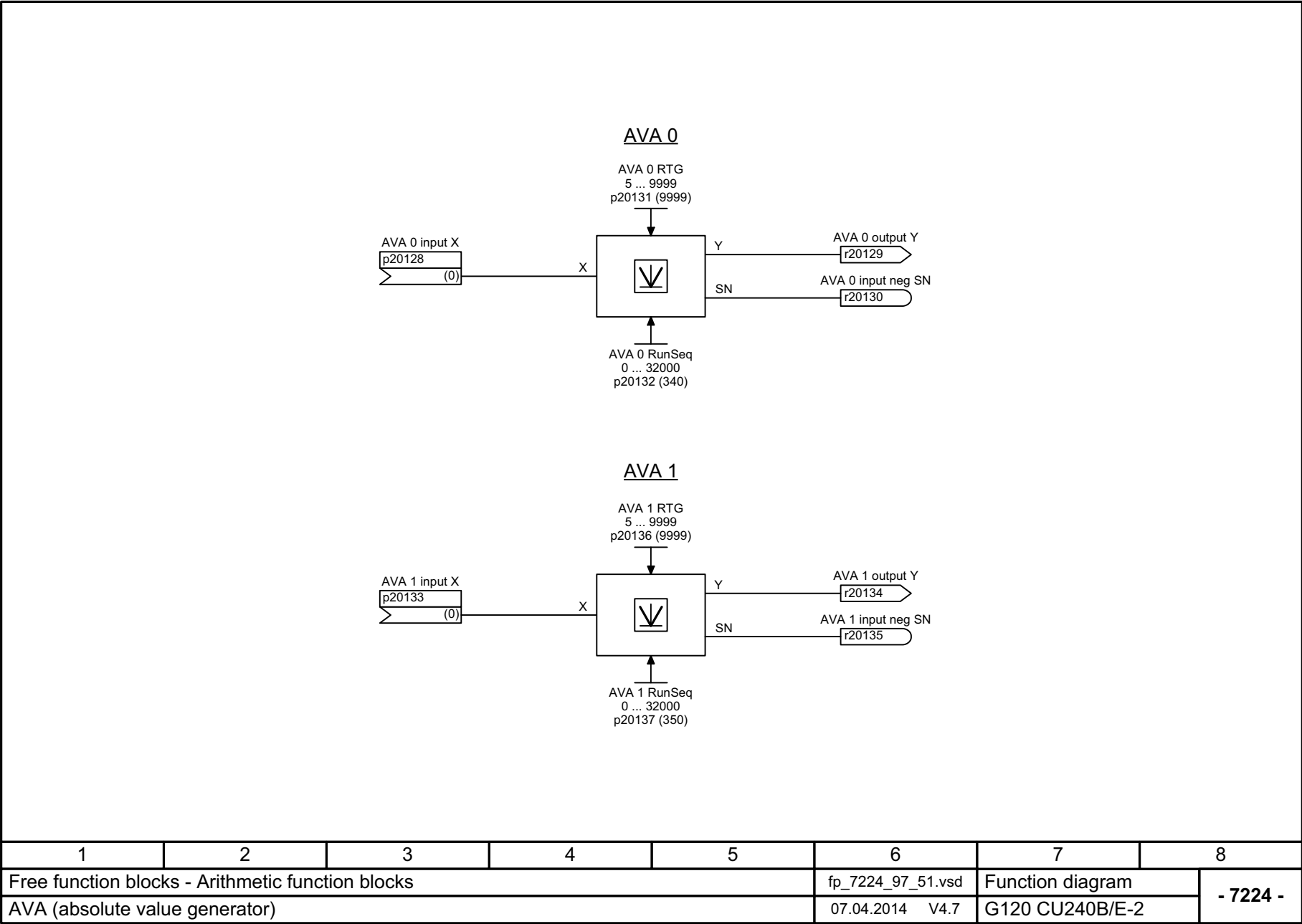
Fig. 3-118 7224 – AVA (absolute value generator)
