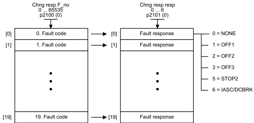
Fig. 3-149 8075 – Faults/alarms configuration
