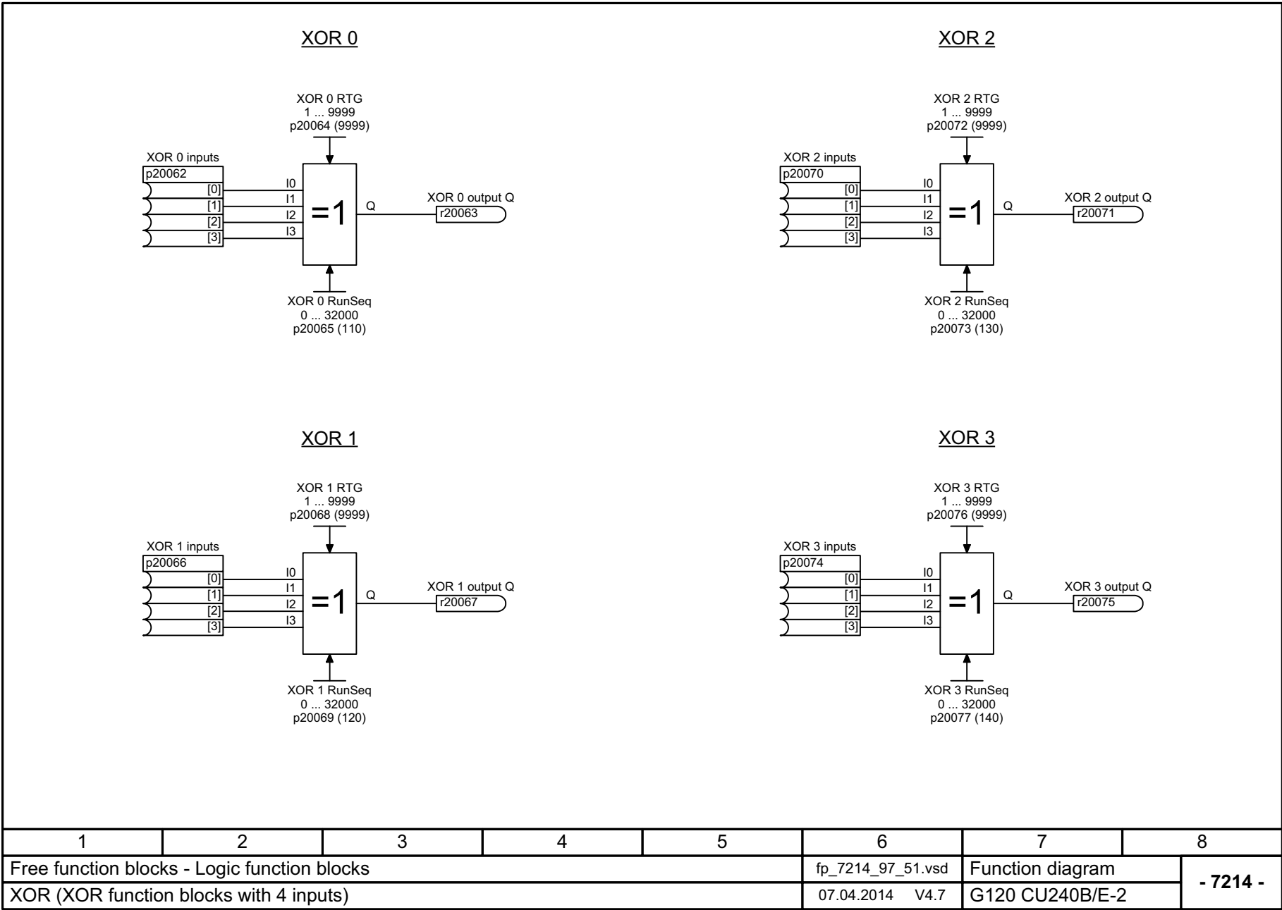
Fig. 3-114 7214 – XOR (XOR function blocks with 4 inputs)
