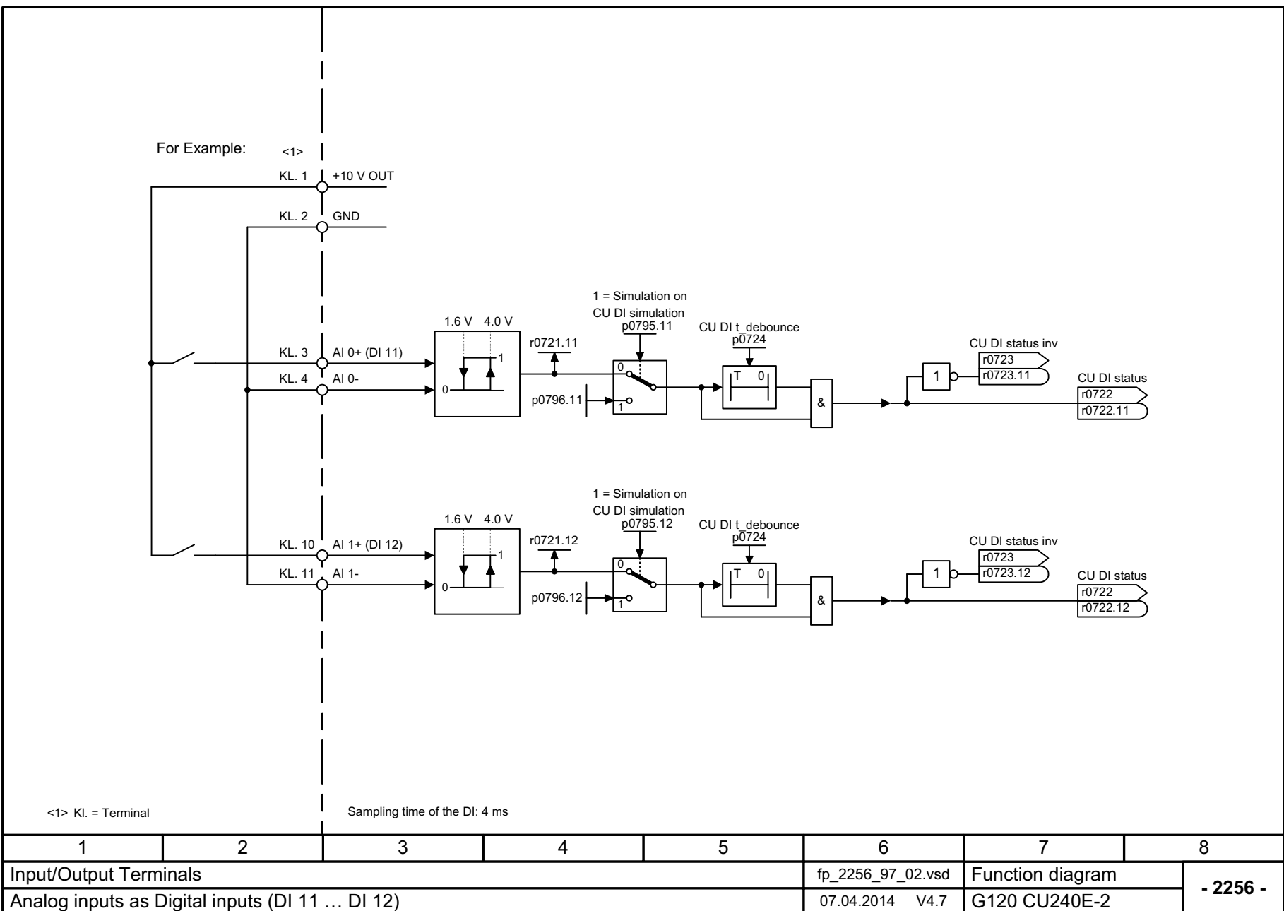
Fig. 3-14 2256 – CU240E-2: Analog inputs as digital inputs (DI 11 ... DI 12)
