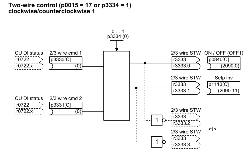
Fig. 3-17 2272 – Two-wire control
