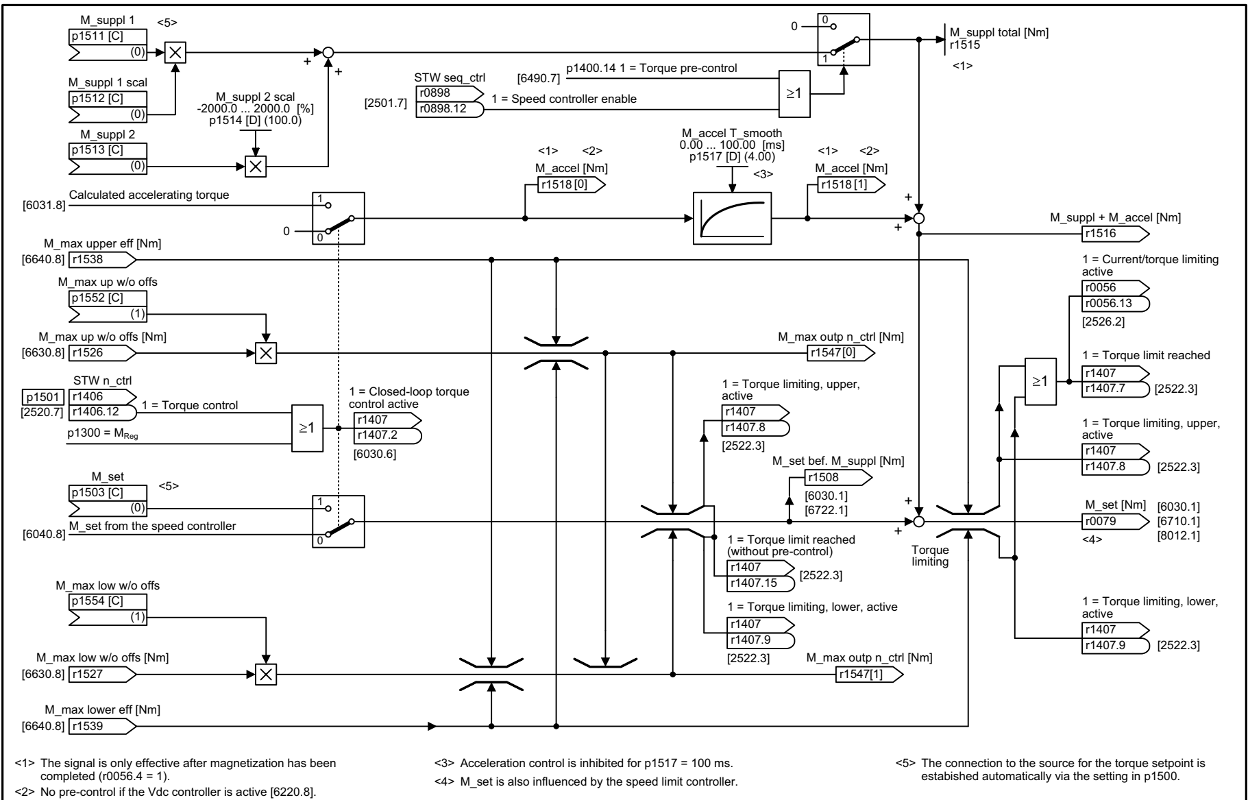
Fig. 3-90 6060 – Torque setpoint
