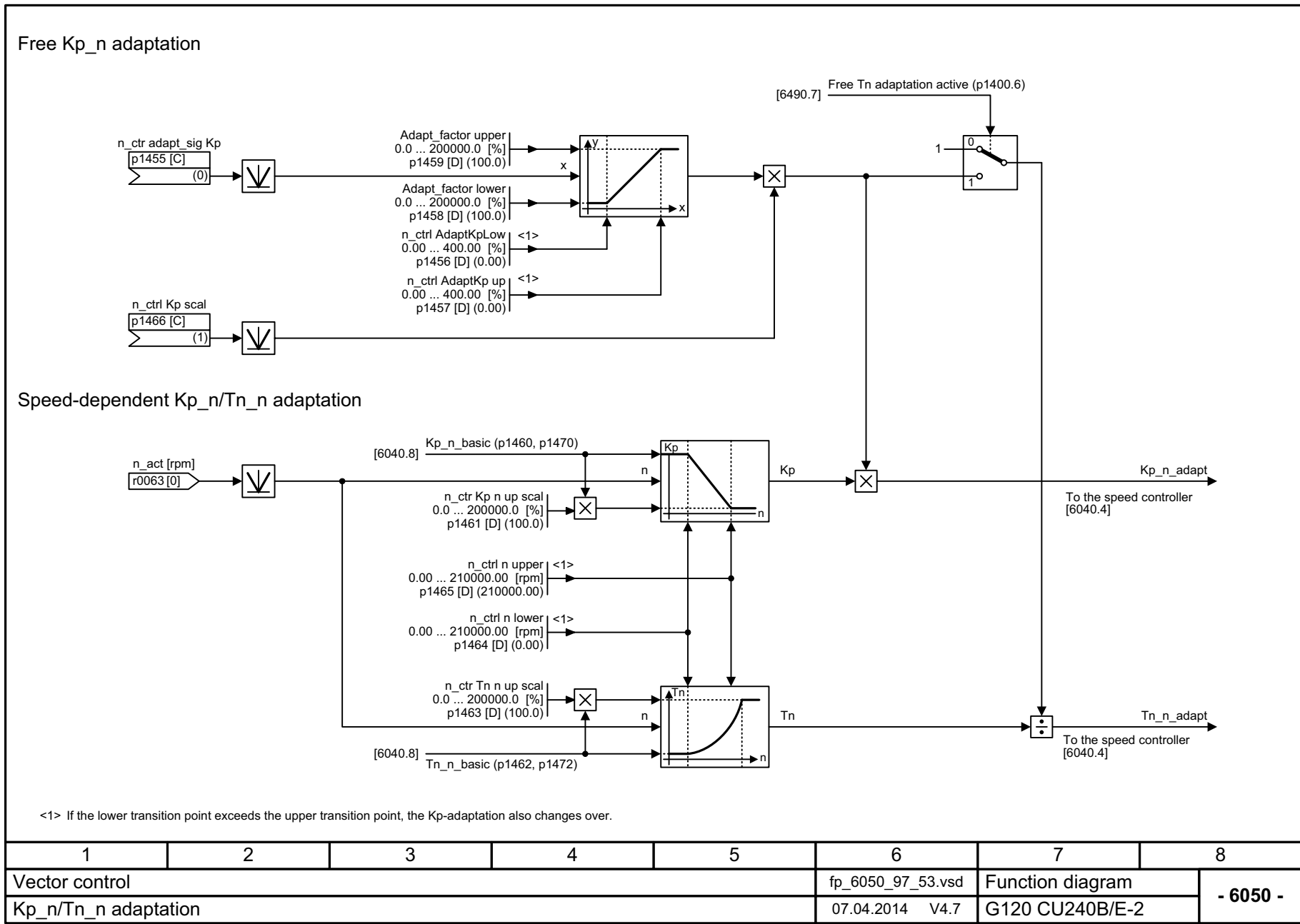
Fig. 3-89 6050 – Kp_n/Tn_n adaptation
