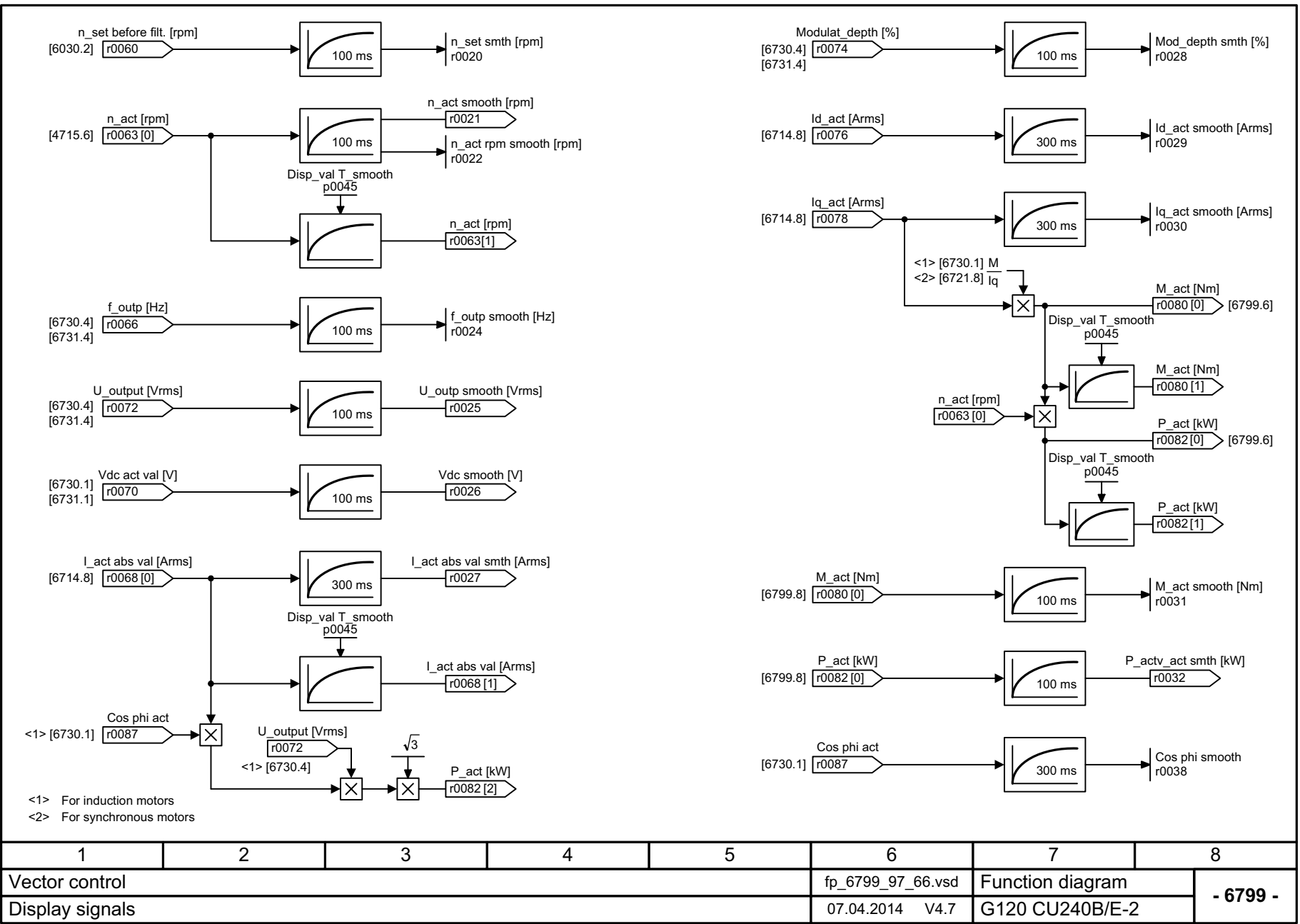
Fig. 3-109 6799 – Display signals
