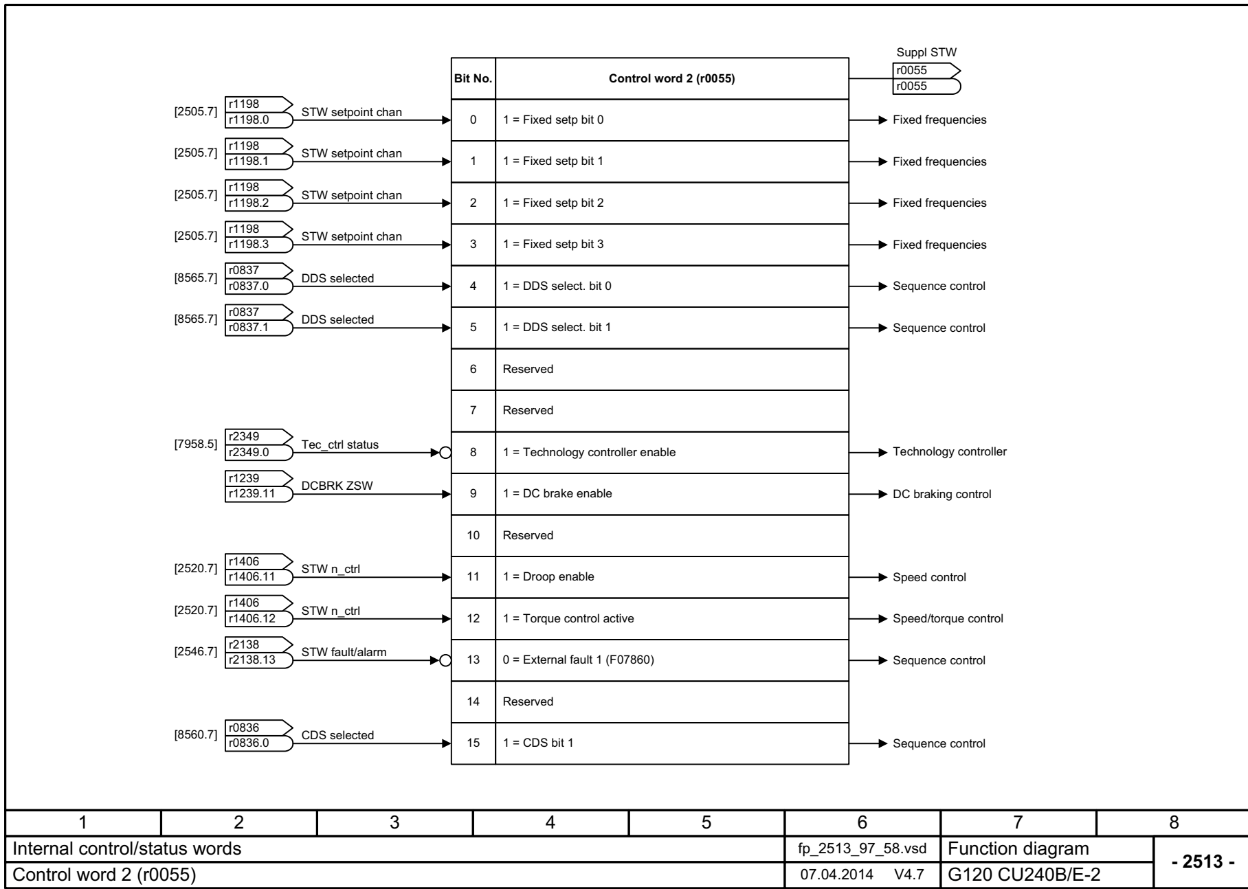
Fig. 3-47 2513 – Control word 2 (r0055)
